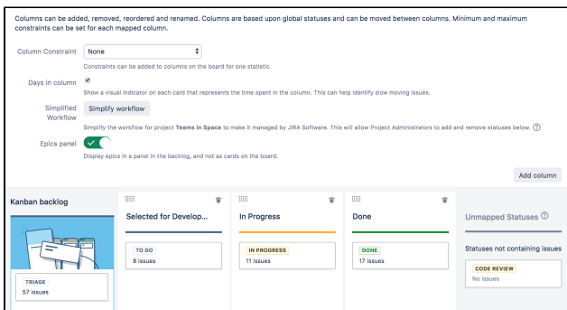
Screenshot: the 'Board Configuration' screen ('Columns' tab) this board is not using Simplified Workflow:
