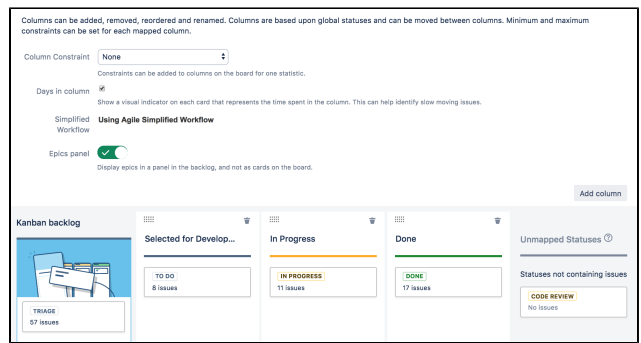
Screenshot: the 'Board Configuration' screen ('Columns' tab) this board is using Simplified Workflow:
